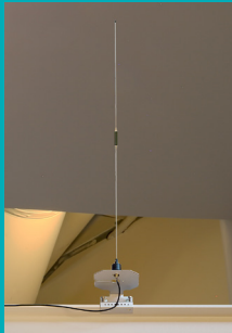
1/2 WAVE WHIPS
